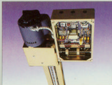
MODULAR BOARD EQUIPPED WITH TIMER, REVERS. SENSOR, & SHUT-OFF SYSTEM.
