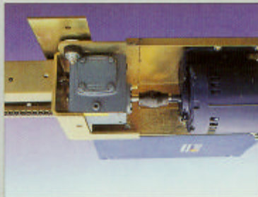
EQUIPPED WITH GEAR BOX & RUBBER ISOLATORS.
